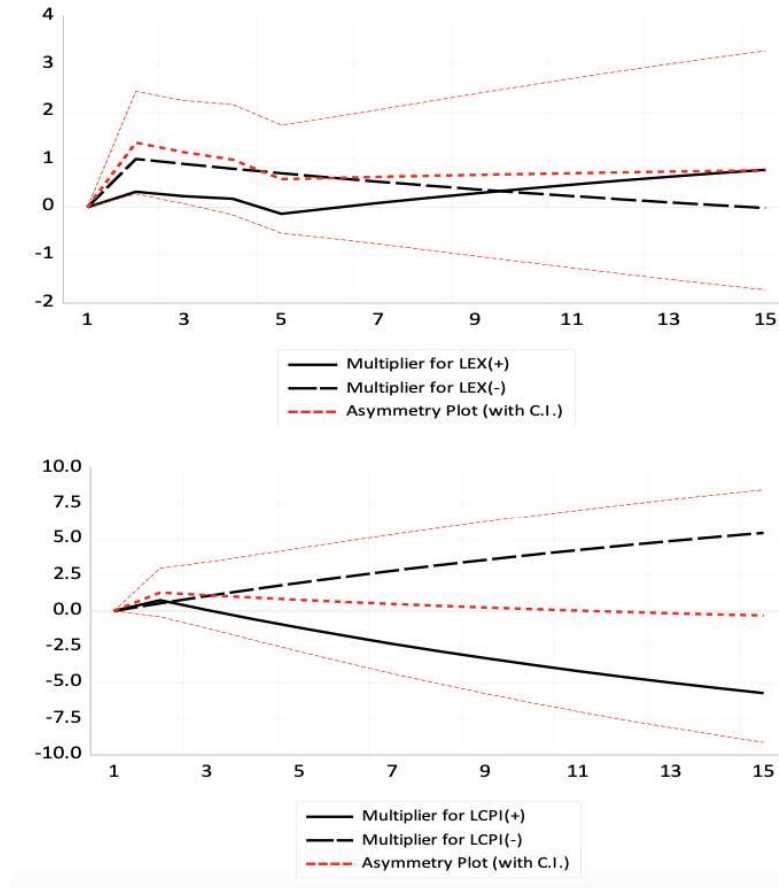
Figure 6: Dynamic multipliers of the NARDL model
