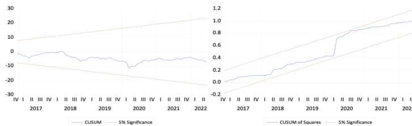
Figure 3: CUSUM and CUSUMSQ of the ARDL model 1
