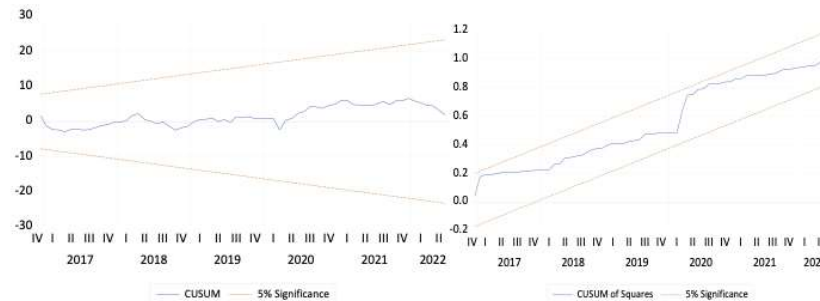
Figure 2: CUSUM and CUSUMSQ of the ARDL model 1
